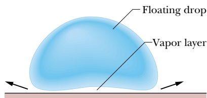
Fig. 4 A Leidenfrost drop in cross section.
