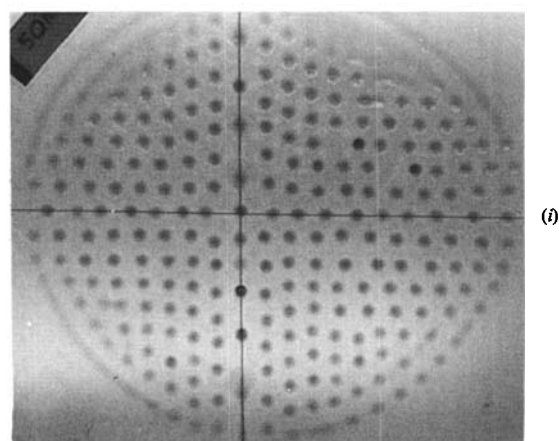
FIGURE 9(a-i). Time evolution of the instability initiated by two wires crossed at 90^\circ . The time interval between two pictures is 360 s. Pairing of two neighbouring peaks is indicated by arrows.
