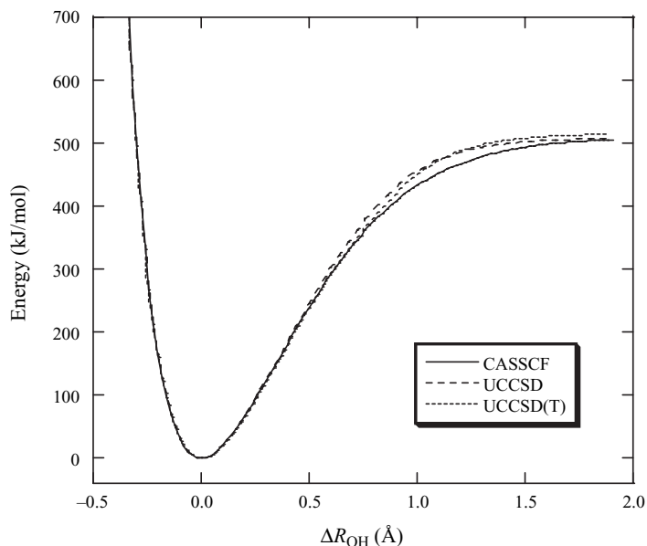
Figure 11.10 UCCSD and UCCSD(T) dissociation curves for \text{H}_2\text{O}
