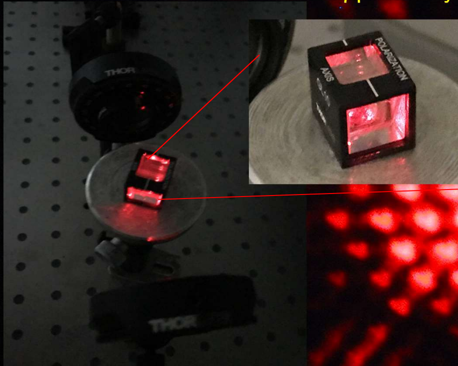
(a) Setup for Polarimetry
