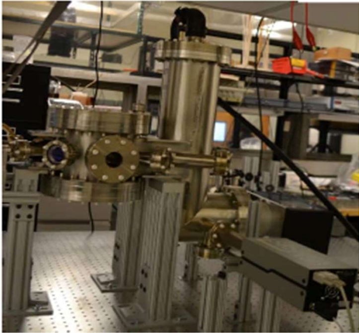
Figure 23. Operating RGA with the ECU on.
