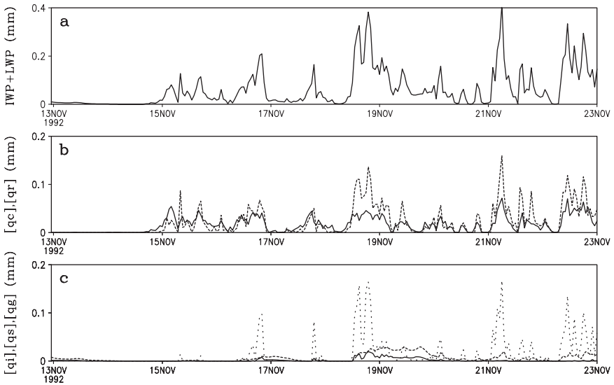
Fig. 6.15 Time series of IWP + LWP in a , [q_c] (solid) and [q_r] (dashed) in b and [q_i] (solid), [q_s] (dashed), and [q_g] (dot) in c simulated in coupled experiment from 13 to 22 November 1992. Unit is mm (After Li 2006)
