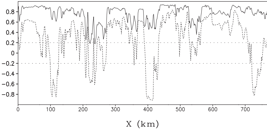
Fig. 10.3 Zonal distribution of linear correlation coefficients between grid-point value and zonal-mean for mixed-layer temperature (dot), salinity (dashed), and depth (solid) in the 2D coupled model simulation. The linear correlation coefficient curves above upper dotted straight line or below lower dotted straight line exceed 95% confidence level (After Li et al. 2000)
