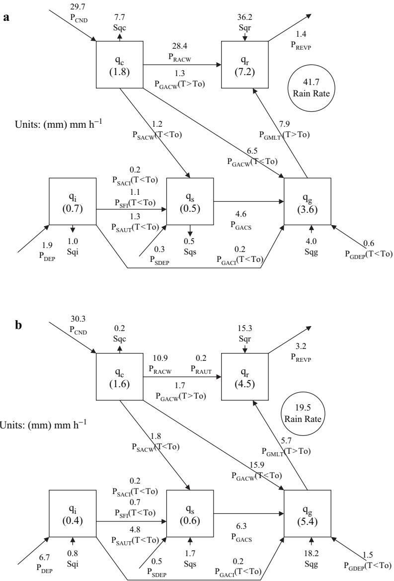
Fig. 6.2 Cloud microphysical budgets averaged within hours 13–15 in a the left half and b the right half of the box in Fig. 4.5. Units for cloud hydrometeor and conversions are mm and mm h -1 , respectively (After Li et al. 2002b)
