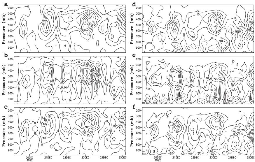
Fig. 3.4 Temporal and vertical distributions of Q_1 for a observation, b COARE1, and c COARE2, and Q_2 for d observation, e COARE1, and f COARE2. Unit is ^\circ\text{C day}^{-1} (After Li et al. 1999)
