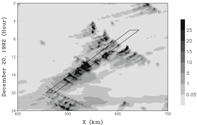
Fig. 4.5 Time evolution and horizontal distribution of surface rain rate ( \text{mm h}^{-1} ) within 400–700 km on 20 December 1992 simulated in COARE. The box between hours 6 and 20 (0600–2000LST) is used to analyze the surface rainfall processes during the life cycle of convection (After Li et al. 2002)
