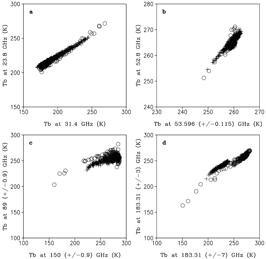
Fig. 12.7 a Brightness temperature T_b at AMSU-A channel 1 (23.8 GHz) versus channel 2 (31.4 GHz), b T_b at AMSU-A channel 4 (52.8 GHz) versus channel 5 [53.596 (+/-0.115) GHz], c T_b at AMSU-B channel 16 [89 (+/-0.9) GHz] versus channel 17 [150 (+/-0.9) GHz], and d T_b at AMSU-B channel 19 [183.31 (+/-3) GHz] versus channel 20 [183.31 (+/-7) GHz]. The dots represent the observations over ( 10^{\circ}\text{S} - 10^{\circ}\text{N} , 140^{\circ}\text{E} - 180^{\circ} ) from NOAA-15 and 16 satellites in selected days of year 2001, whereas the crosses denote the simulations from microwave radiative transfer model developed by Liu and Weng (2002). The simulations use cloud information in COARE from 2200 LST 19 December to 1000 LST 21 December 1992. The simulation data are averaged in 32 grid points (48 km mean), which is similar to the horizontal resolution of AMSU observation at nadir. All data are obtained in cloudy condition in which vertically integrated cloud water is larger than 0.1 mm (After Li and Weng 2003). The cloud data are from experiment COARE
