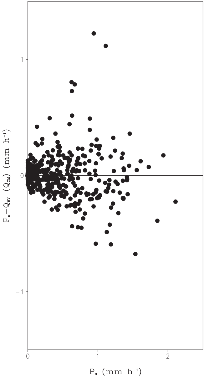
Fig. 4.3 Zonal-mean Q_{CM} ( P_s - Q_{WV} ) versus zonal-mean P_s in COARE ( \text{mm h}^{-1} ) (After Gao et al. 2005)
