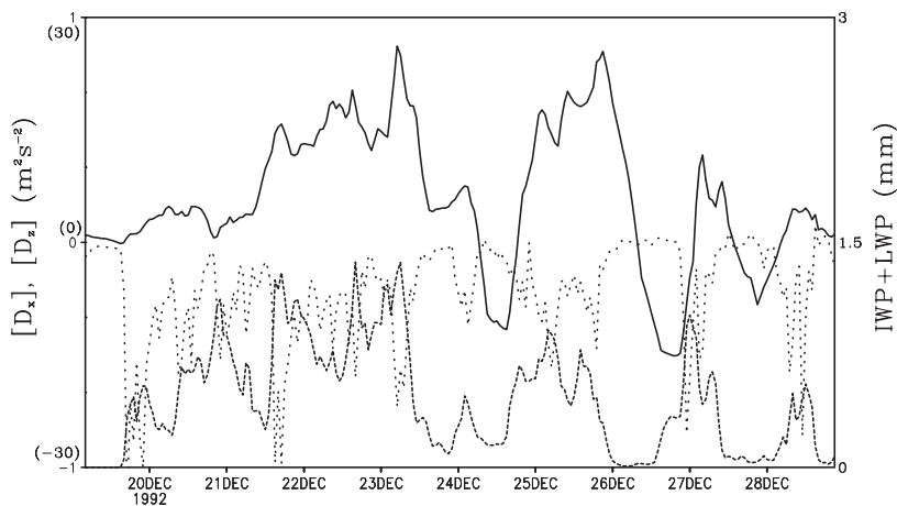
Fig. 7.6 Time series of [D_x] ( \text{m}^2 \text{s}^{-2} , dotted line), [D_z] ( \text{m}^2 \text{s}^{-2} , solid line) and IWP + LWP (mm, dashed line) in the 10-day 2D cloud-resolving model simulation during TOGA COARE. The plotting scales of [D_x] , [D_z] , and IWP + LWP are -1 - 1 \text{ m}^2 \text{ s}^{-2} , -30 - 30 \text{ m}^2 \text{ s}^{-2} , and 0-3 \text{ mm} , respectively (After Gao et al. 2005)
