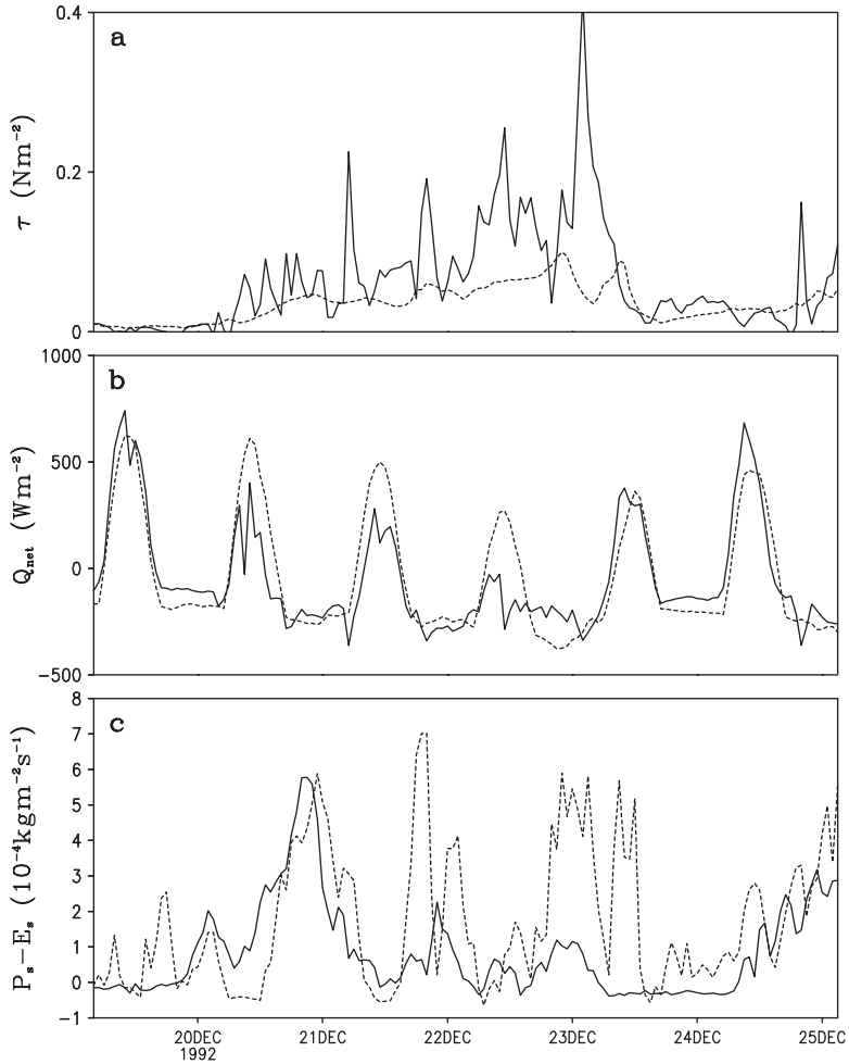
Fig. 3.7 Time series of a zonal-mean zonal wind stress ( \text{N m}^{-2} ), b net surface heat fluxes ( \text{W m}^{-2} ), and c fresh water flux ( 10^{-4} \text{kg m}^{-2} \text{s}^{-1} ) observed during TOGA COARE (solid) and simulated in the 2D coupled ocean-cloud-resolving atmosphere model (dashed) with the forcing from TOGA COARE (see Fig. 3.1a) (After Li et al. 2000)
