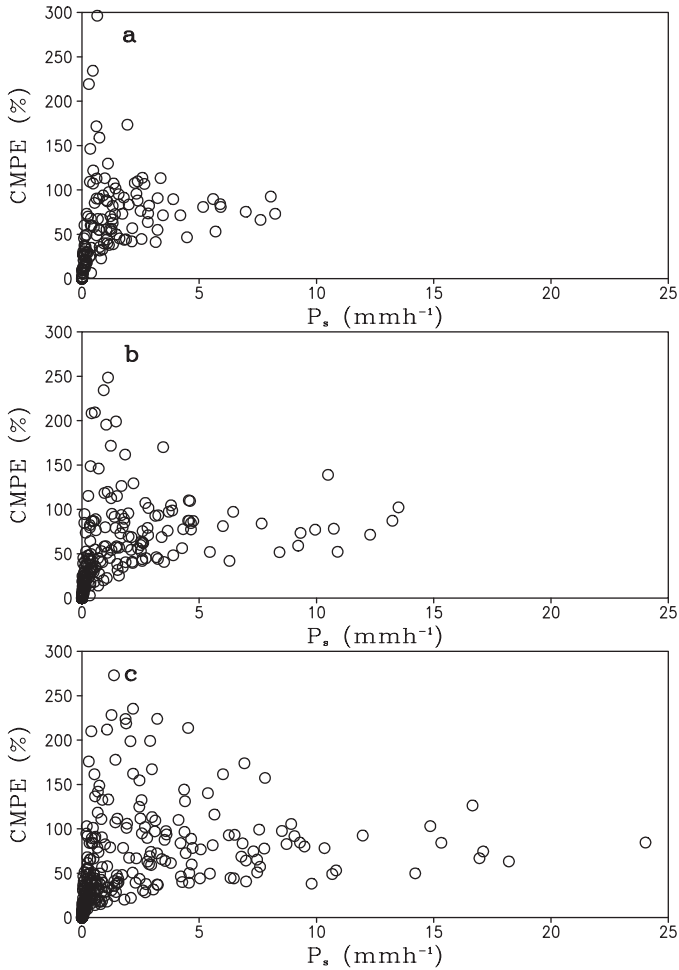
Fig. 9.6 CMPE (%) versus P_s (mm h -1 ) averaged within a 96 km, b 48 km, and c 24 km in COARE (After Sui et al. 2005)
