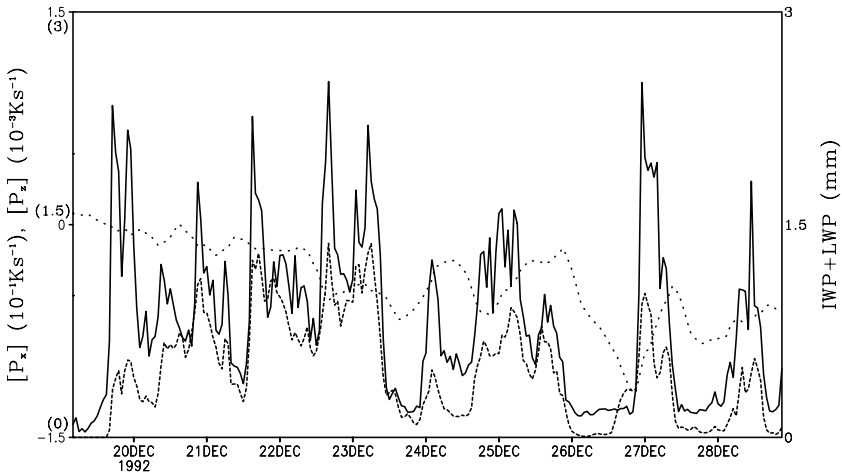
Fig. 7.1 Time series of zonally averaged, mass-integrated zonal ( [P_x] , 10^{-1} \text{ K s}^{-1} , dot line) and vertical ( [P_z] , 10^{-3} \text{ K s}^{-1} , solid line) components of the 2D CVV , and IWP + LWP (mm, dashed line) in the 10-day 2D cloud-resolving model simulation during TOGA COARE. The plotting scales of [P_x] and [P_z] and IWP + LWP are -0.15 - 0.15 \text{ K s}^{-1} , 0 - 3 \times 10^{-3} \text{ K s}^{-1} , and 0 - 3 \text{ mm} , respectively (Gao et al. 2004)
