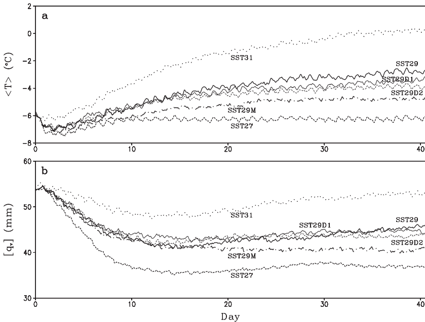
Fig. 11.1 Time series of a zonal- and mass-weighted mean temperature ( ^\circ\text{C} ) and b zonal-mean PW (mm) in SST27 (dark dashed), SST29 (dark solid), SST31 (dot), SST29M (dark dot dashed), SST29D1 (light solid), and SST29D2 (light dashed) (After Gao et al. 2007)
