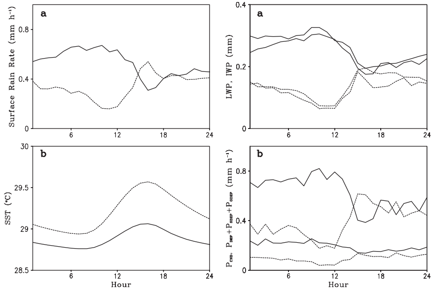
Fig. 8.5 Left panel: diurnal composites of a P_s ( \text{mm h}^{-1} ) and b SST ( ^{\circ}\text{C} ). Right panel: diurnal composites of a LWP (dark) and IWP (light) (mm) and b P_{\text{CND}} (dark) and sum of P_{\text{DEP}} , P_{\text{SDEP}} , and P_{\text{GDEP}} (light) ( \text{mm h}^{-1} ). Solid and dashed lines denote cases W and S in the coupled model simulation, respectively (After Gao et al. 2006)
