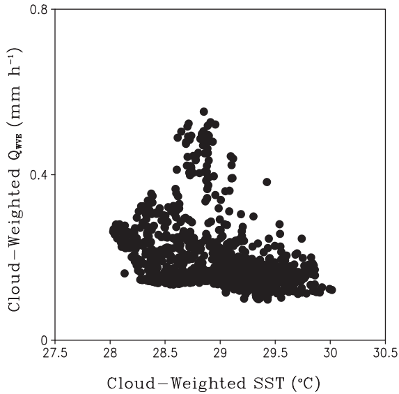
Fig. 10.5 Cloud-weighted Q_{WVE} versus cloud-weighted SST ( ^{\circ}C ) (After Gao et al. 2006)
